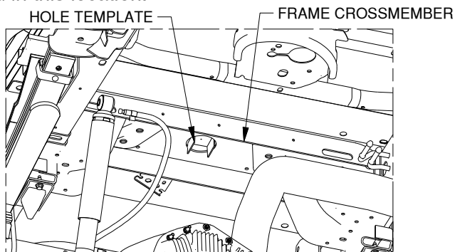
Figure A4: View under bed looking towards the cab.
