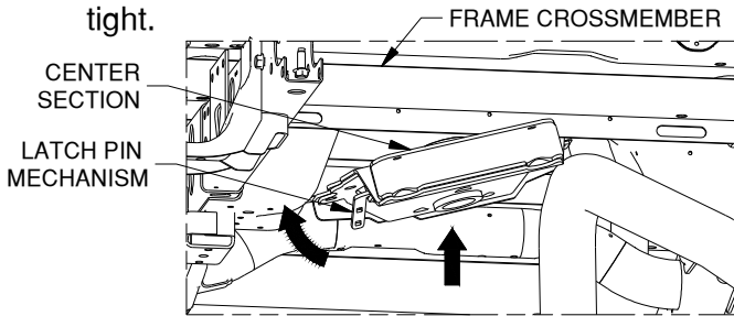
Figure B4: Looking from rear towards cab.
