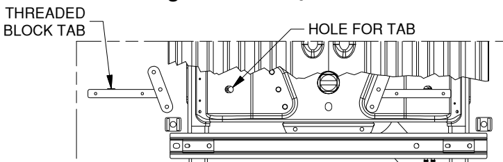
Figure B4: Cutaway view looking down into bed.
