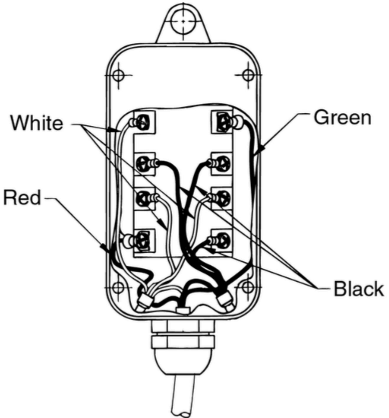
4 - Wire Cord (4 Way) Terminal Connections
